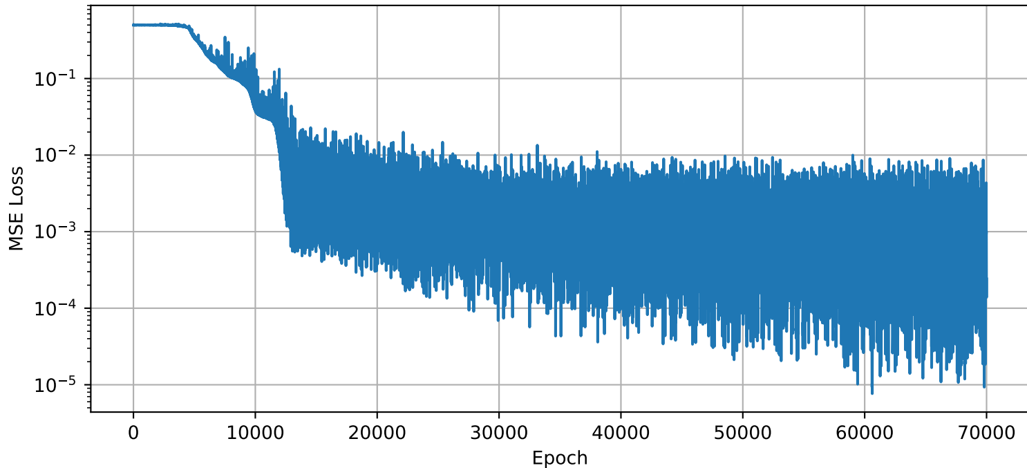
Training Loss
