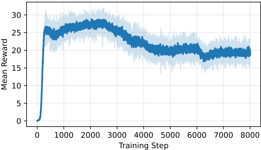
Train/mean_reward
