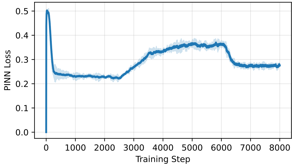
Loss/pinn_loss
