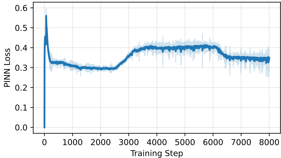
PINN Loss
