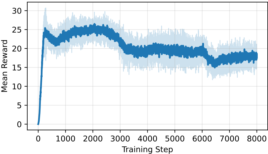
Mean Reward
