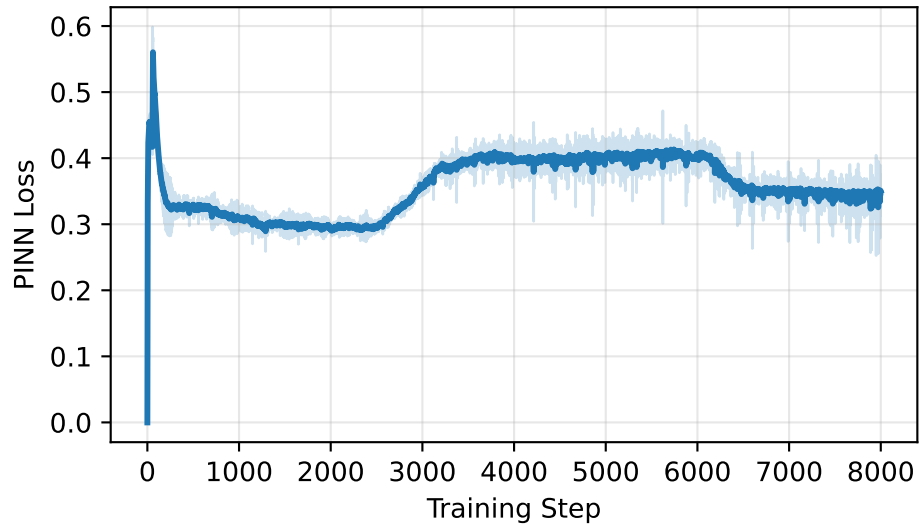
PINN Loss
