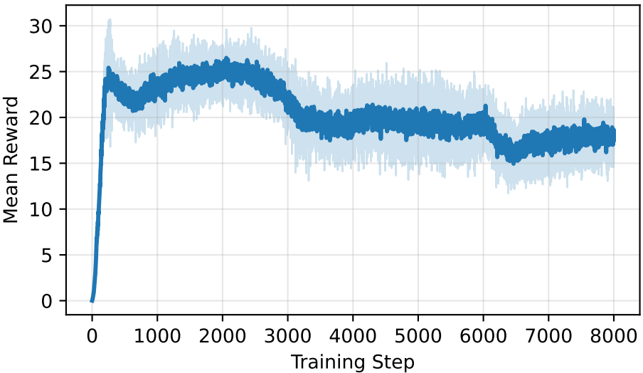
Mean Reward
