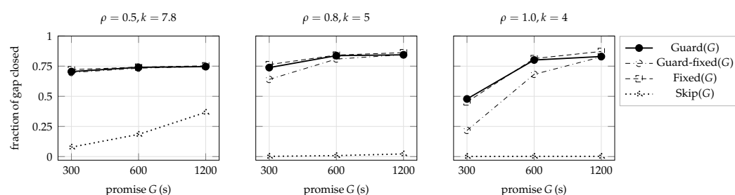
Figure 3. What each budget shape keeps of the FCFS-to-SJF gap as the promised excess G is relaxed. Every point is a “Gap closed” cell of Table 8; the intervals are in that table and are omitted here. All four policies carry the same promise at a given G , since the promise depends on the cap alone. The gap between Guard( G ) and its constant-shape ablation opens where the promise is tight and the load is high and closes elsewhere; counting positions rather than work (Skip) collapses at the two higher loads; Fixed( G ), which spends the whole cap, buys its gap with harm the selection rule rejects.
