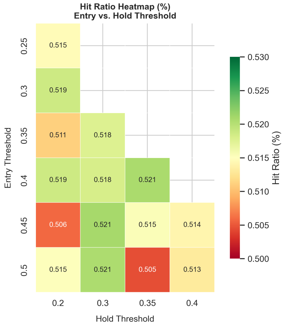
Figure 5.14: Performance of the hysteresis strategy as a function of the hold and entry threshold on the American equity data set from 1990 to 2020 with an initial capital of 100. The performance is measured as the combination of hit ratio and win/loss ratio.
