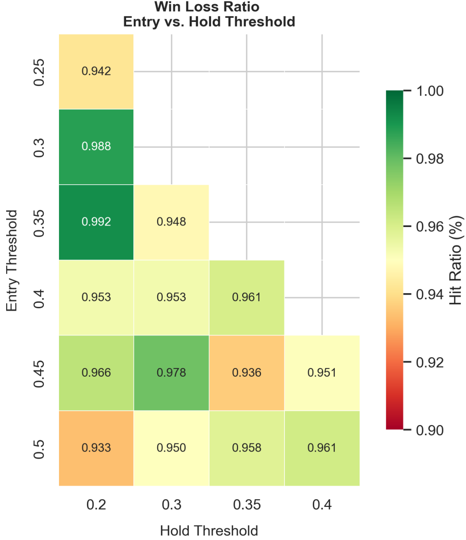
Figure 19: Performance of the hysteresis strategy as a function of the hold and entry threshold on the American equity data set from 1990 to 2020 with an initial capital of 100. The performance is measured as the combination of hit ratio and win/loss ratio.
