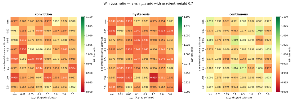
Figure 16: Performance in terms of win loss ratio of the implied probability strategy as a function of the temperature parameters \tau and \tau_{grad} on the American equity data set from 1990 to 2020 with an initial capital of 100.
