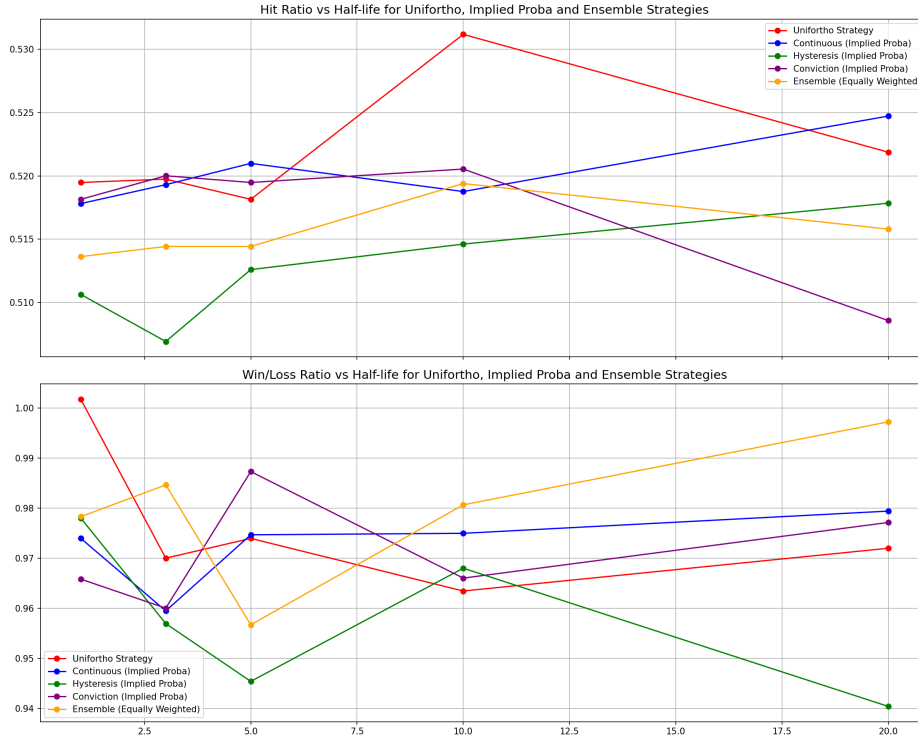
Figure 17: Performance of the equally weighted ensemble method as a function of the half-life parameter \lambda on the American equity data set from 1990 to 2020 with an initial capital of 100. The performance is measured as the combination of hit ratio and win/loss ratio.
