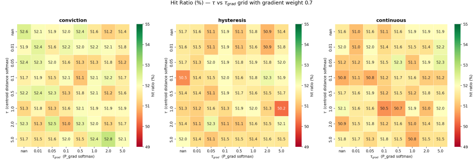
Figure 15: Performance in terms of hit ratio of the implied probability strategy as a function of the temperature parameters \tau and \tau_{grad} on the American equity data set from 1990 to 2020 with an initial capital of 100.
