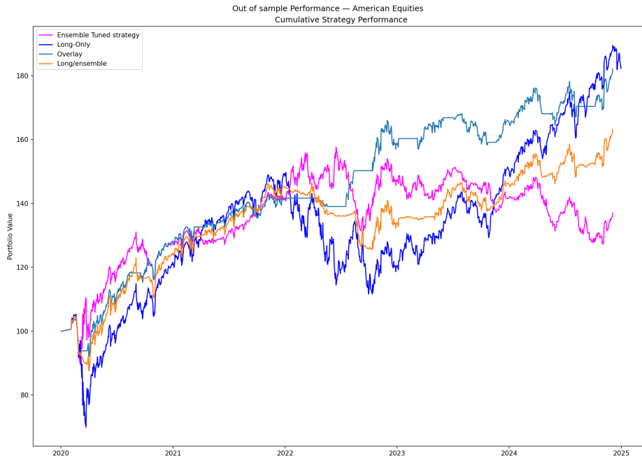
Figure 20: Out-of-sample performance of the equally weighted ensemble method with \alpha = 0.6 on the American equity data set from 1st of January 2020 to 31st of December 2024 with an initial capital of 100.
