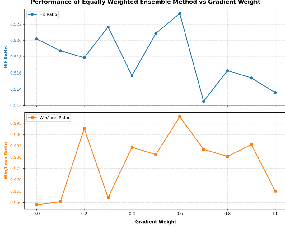
Figure 14: Performance of the equally weighted ensemble method as a function of the gradient weight \alpha on the American equity data set from 1990 to 2020 with an initial capital of 100. The performance is measured as the combination of hit ratio and win/loss ratio.
