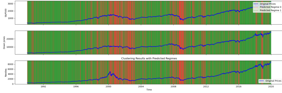
Figure 5: Regime labels output by the Sliced-Wasserstein k-means clustering algorithm with UnifOrtho projections on the US equity indices (S&P 500, NASDAQ, Dow Jones) time series. Parameters h_1 = 3 , h_2 = 1 , L = 20 , N_S = 40 .
