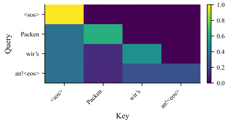
S1: decoder self-attn
