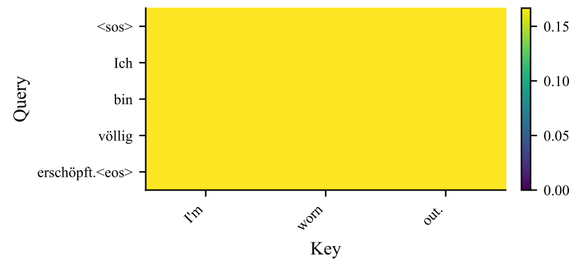
S4: decoder cross-attn
