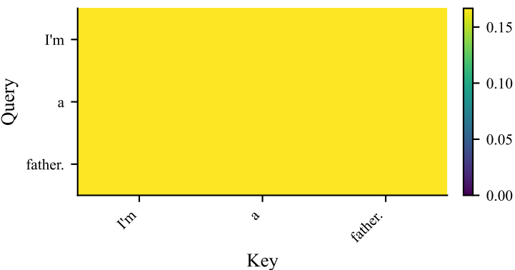
S3: encoder self-attn
