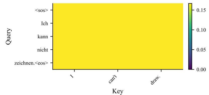
S2: decoder cross-attn
