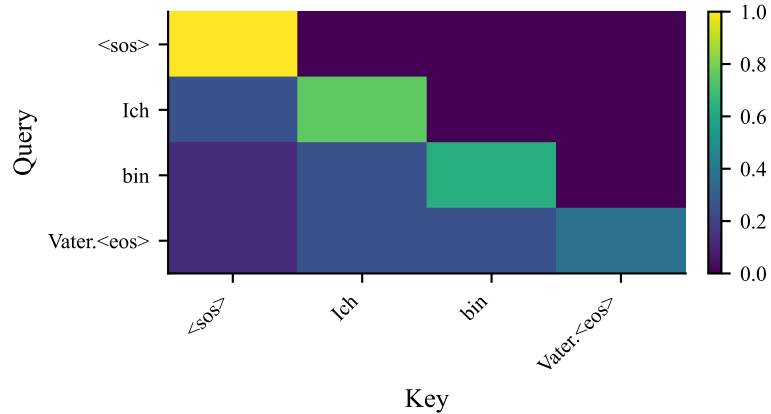
S3: decoder self-attn
