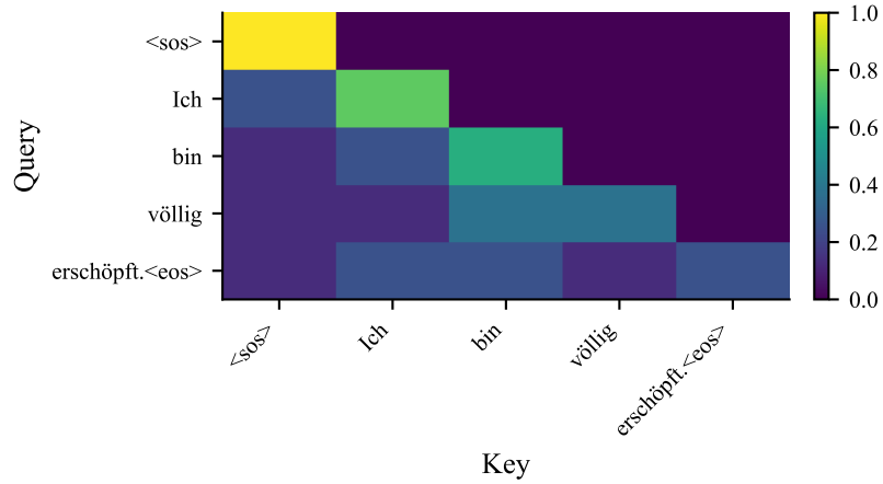
S4: decoder self-attn
