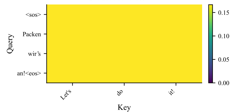
S1: decoder cross-attn
