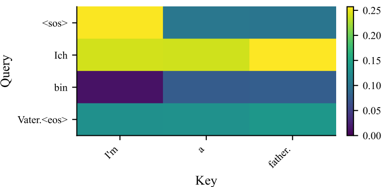
S3: decoder cross-attn
