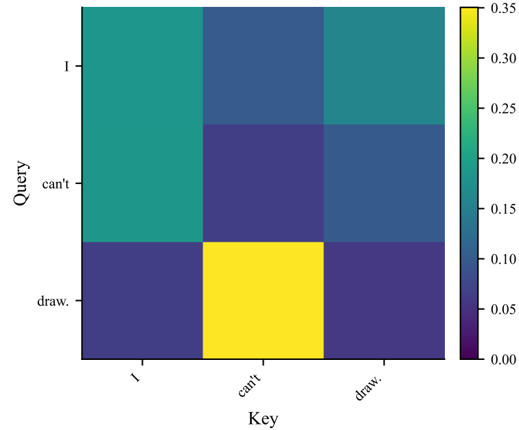
Encoder self-attn (L4)
