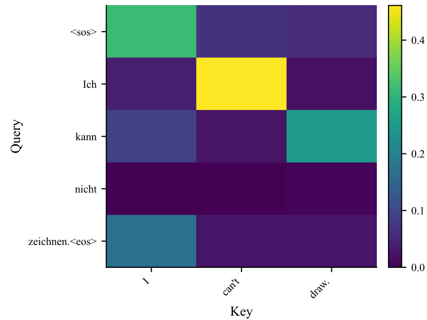
Decoder cross-attn (L4)
