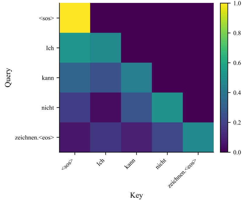
Decoder self-attn (L4)
