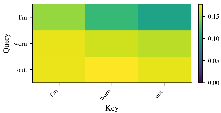
S4: encoder self-attn
