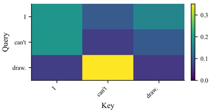
S2: encoder self-attn
