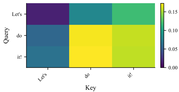
S1: encoder self-attn
