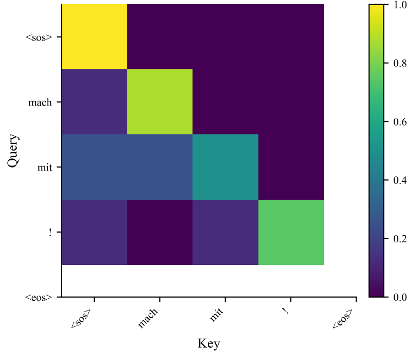
Decoder self-attn (L4)
