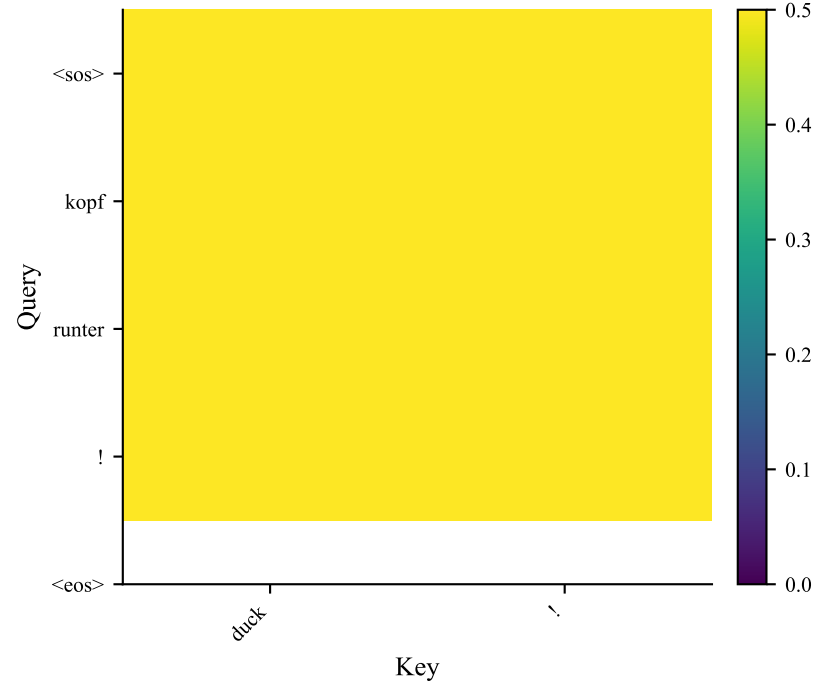
Decoder cross-attn (L4)
