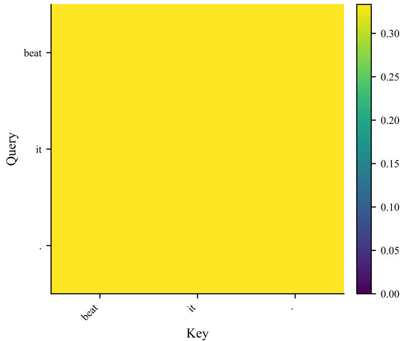
Encoder self-attn (L4)
