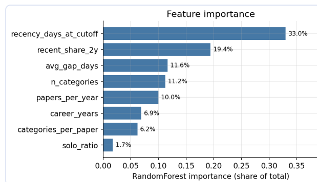
Fig E • RandomForest importance. Recency (33%) and recent-output share (19%) dominate the model — the quantitative echo of the four selection methods and of the unit's motto.
