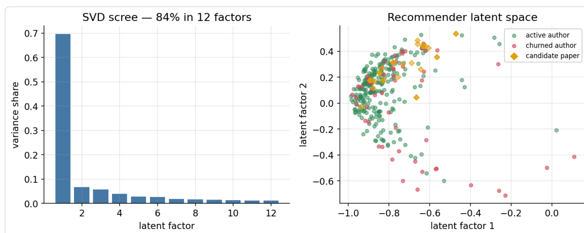
Fig C · SVD of the researcher \times category matrix ( scipy.sparse.linalg.svds , k=12 , 84% variance). Left : scree — the first factor alone holds \sim 70\% of the structure. Right : authors (circles, by churn) and candidate papers (gold) in the recommender's latent space; proximity = shared research interest, which is exactly how recommendations are chosen.
