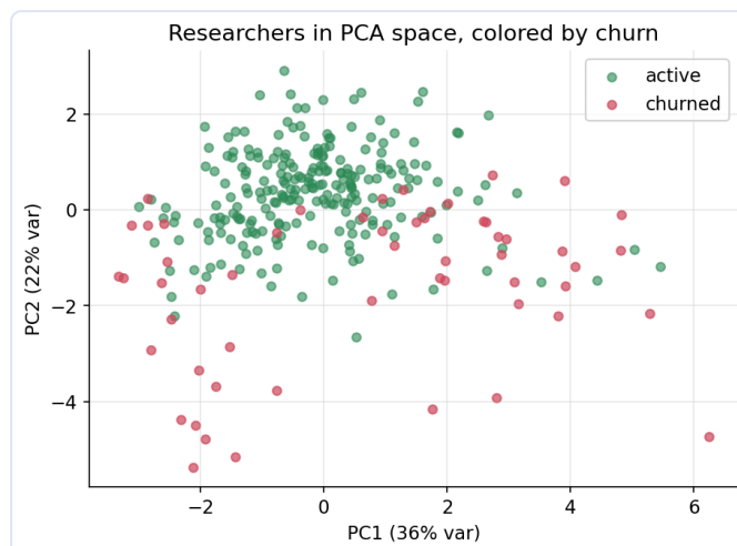
Fig B · PCA churn map. The 295 researchers projected to 2D, colored by churn. Red (churned) separates from green (active) along PC1 (recency) — visible separation is the proof the engineered features carry real signal.
