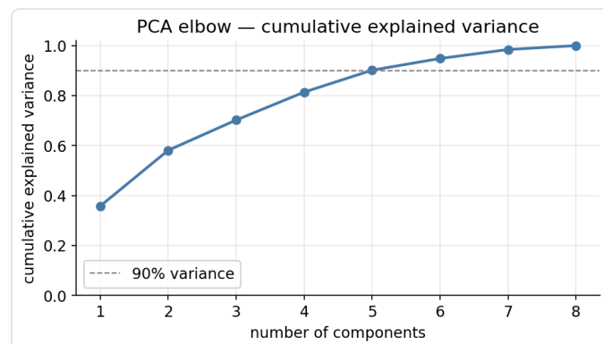
Fig A · PCA elbow. Cumulative explained variance vs number of components: 2 components capture \approx 58\% , 3 \approx 70\% . The curve justifies keeping few components for visualization.
