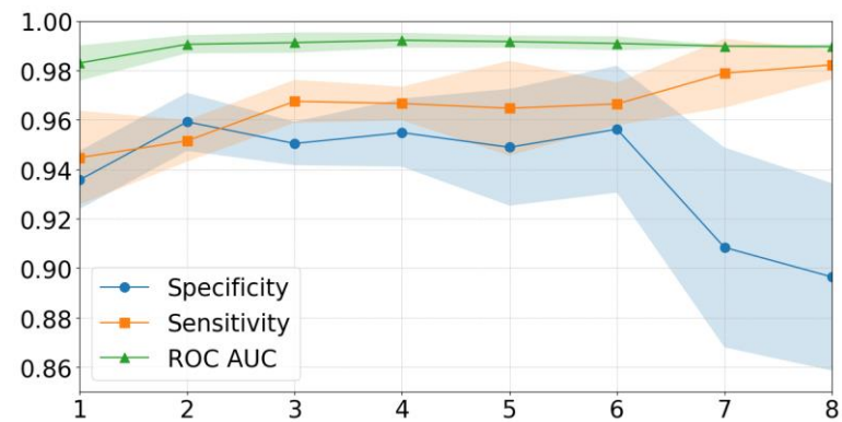
RNN-based architecture
