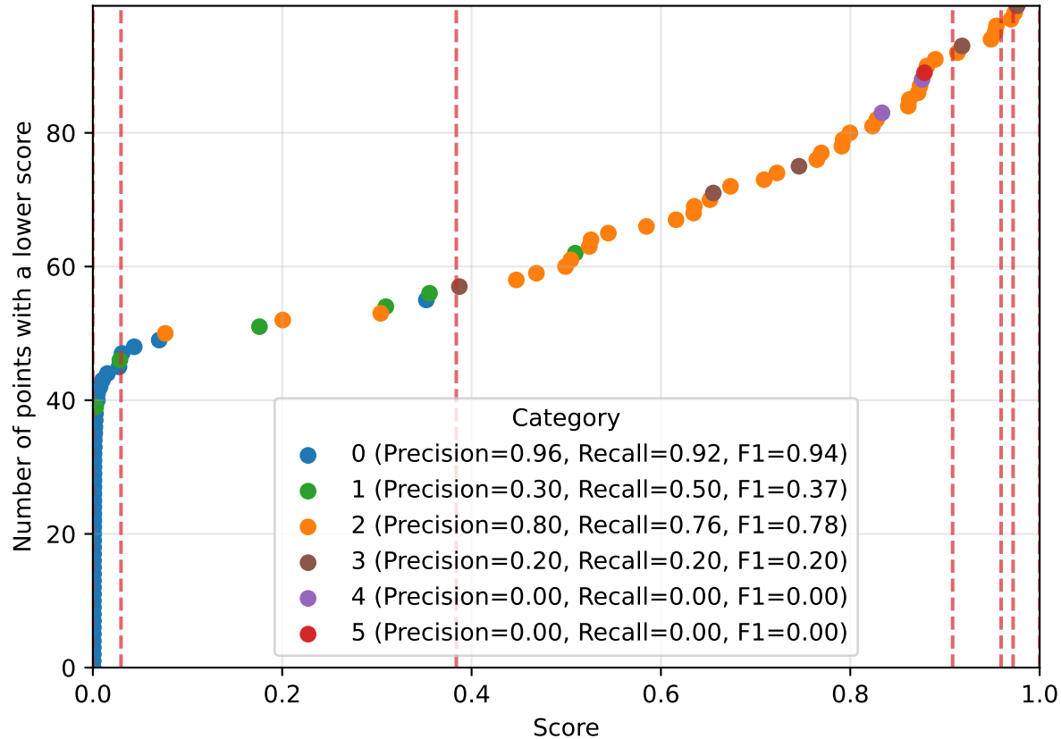
Cumulative count by category: Llama2 on JailbreakBench -- Finetune average quantiles
