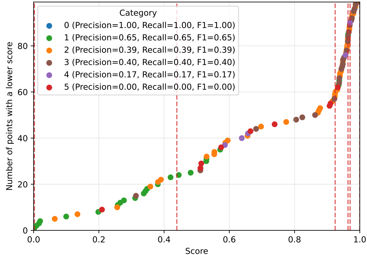
Cumulative count by category: Vicuna on JailbreakBench -- Finetune
