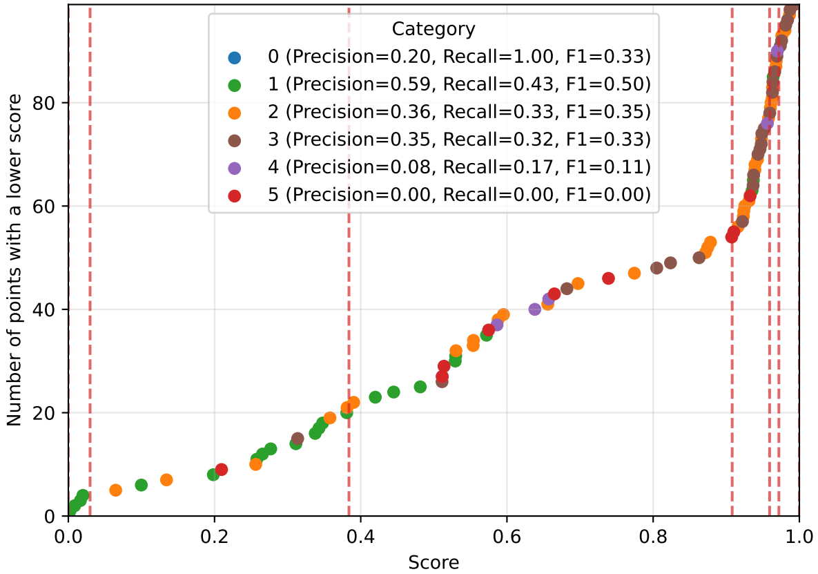
Cumulative count by category: Vicuna on JailbreakBench -- Finetune average quantiles
