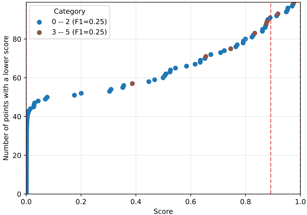
Cumulative count by category: Llama2 on JailbreakBench -- Finetune
