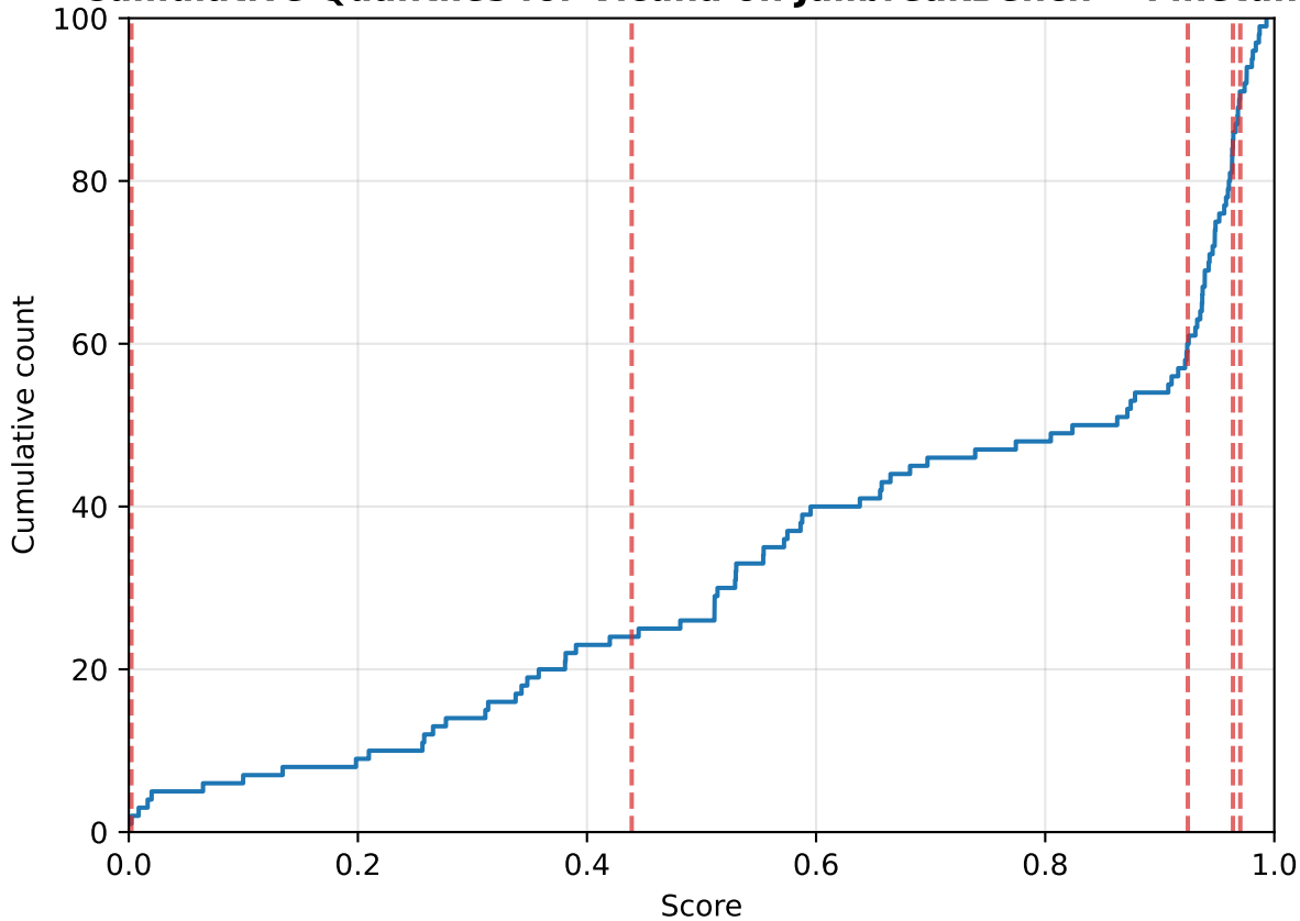
Cumulative Quantiles for Vicuna on JailbreakBench -- Finetune
