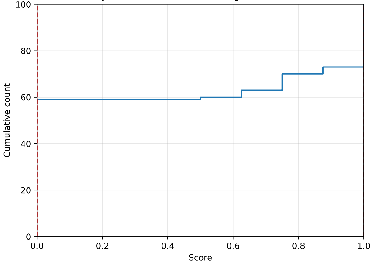
Cumulative Quantiles for Llama2 on JailbreakBench -- Rubric
