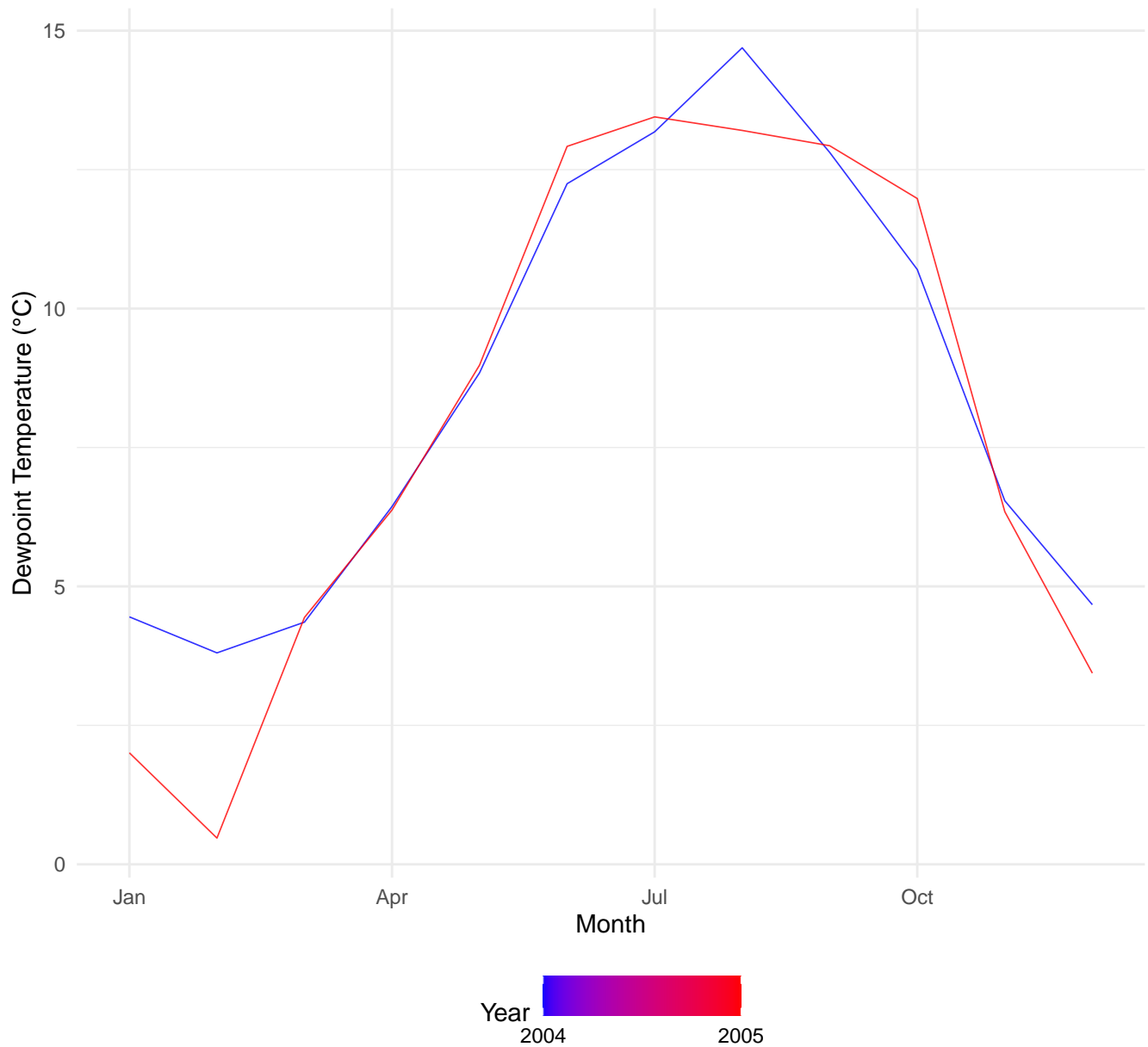
Time Series of Dewpoint Temperature (°C)
