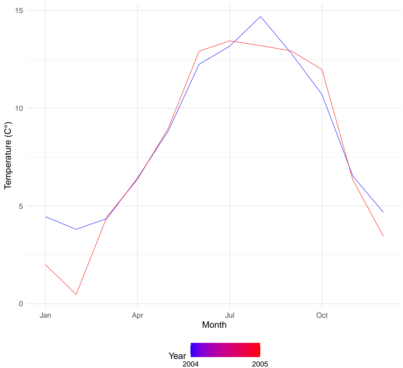
Time Series of Temperature (C°)
