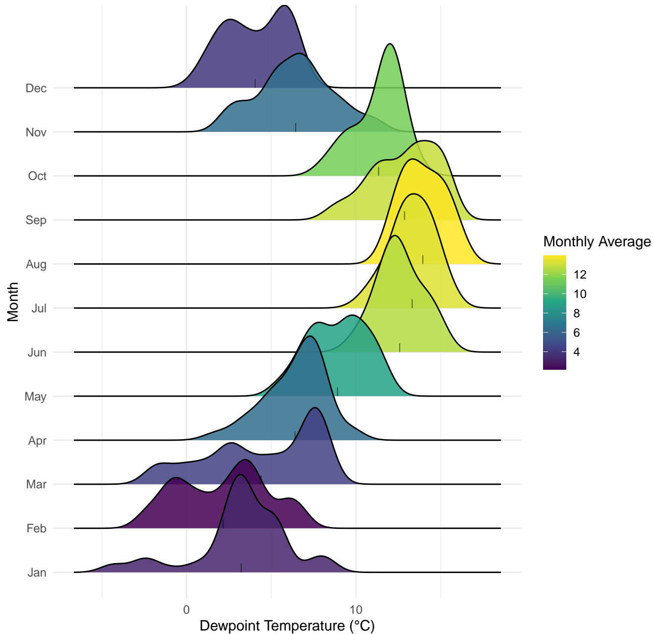
Distribution of Dewpoint Temperature (°C) by Month
