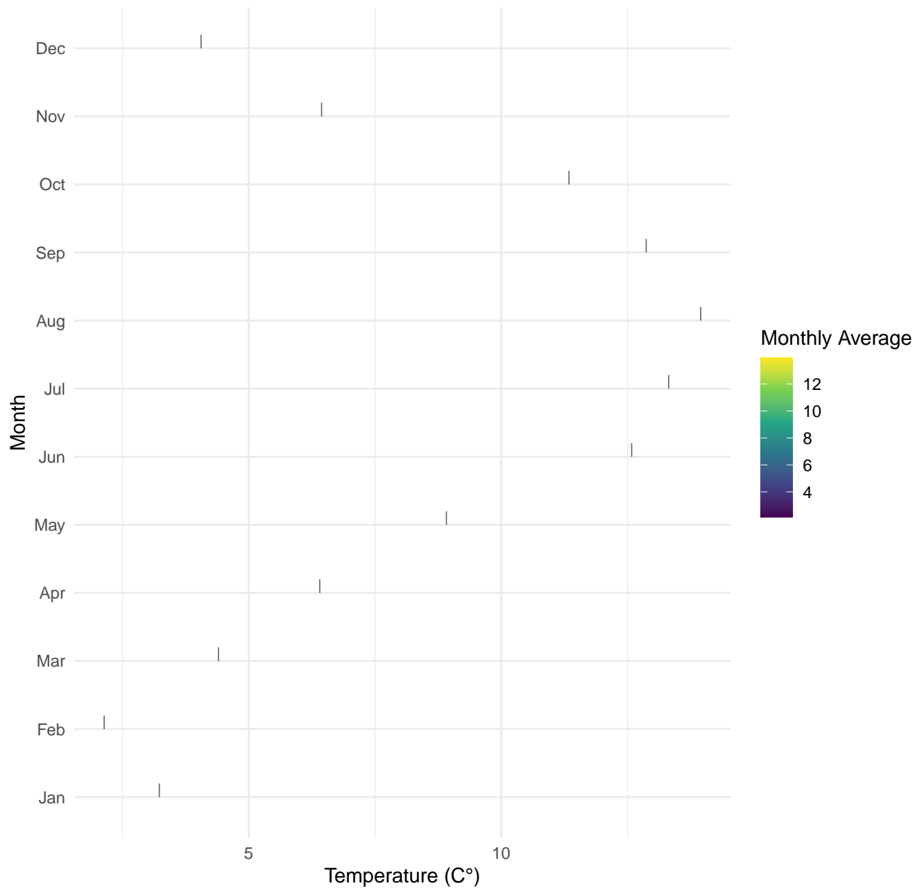
Distribution of Temperature (C°) by Month
