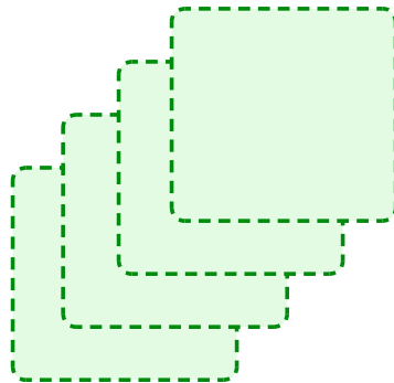
Chunks Grandes
