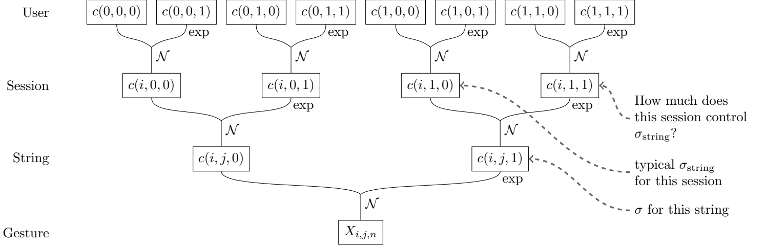
Figure 6.1: A hierarchical temporal model in which user-level statistics refine through session- and string-level variables to individual gestures.
