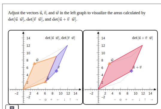
Figure 12.28 DoenetML example
