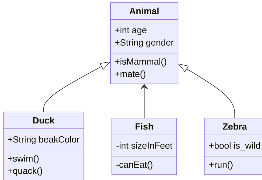
Figure 10.23 Mermaid Class Diagram
