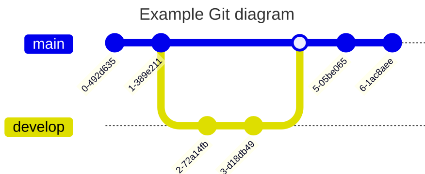
Figure 10.22 Mermaid Git Diagram
