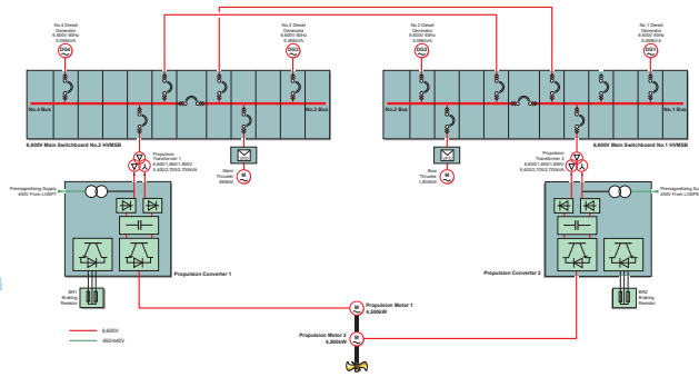
(b) Propulsion System
