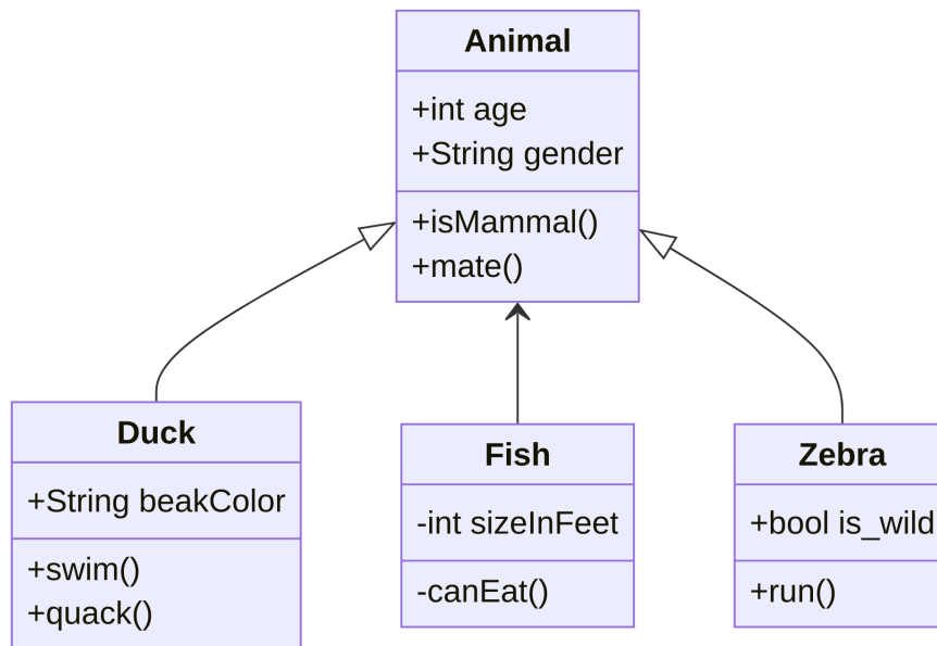
Figure 10.23 Mermaid Class Diagram
