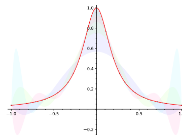
Figure 10.30 Sage polynomial approximations of f(x) = 1/(1 + 25x^2)
