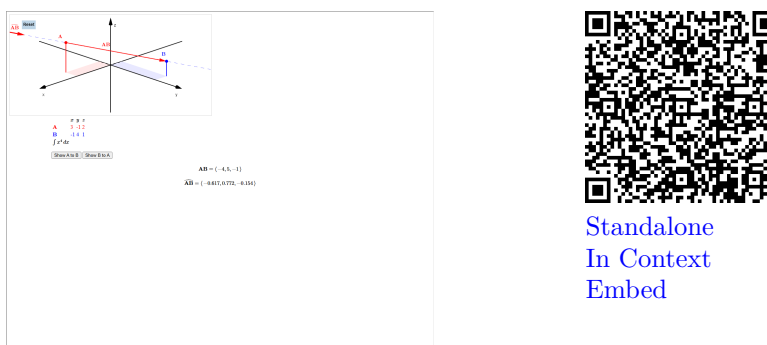
Figure 14.27 Geogebra/PreTeXt Communications
