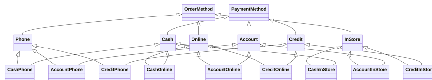
Figure 10.25 Mermaid Class Diagram using ELK layout engine
