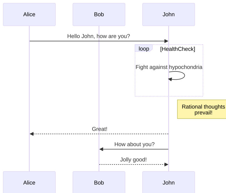
Figure 10.24 Mermaid Sequence Diagram
