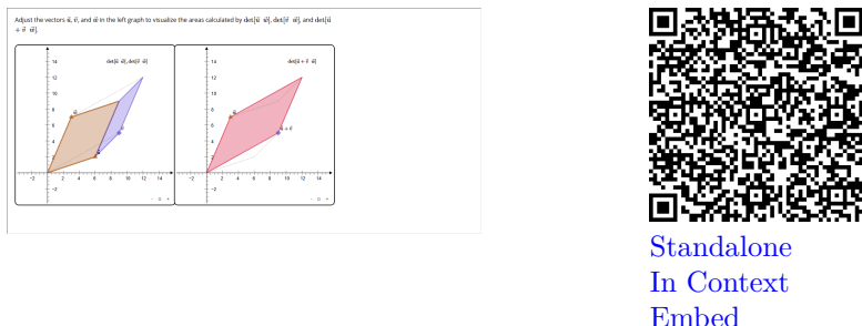
Figure 14.34 DoenetML example
