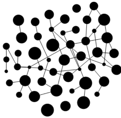
Figure 14.8 Graph Layout
