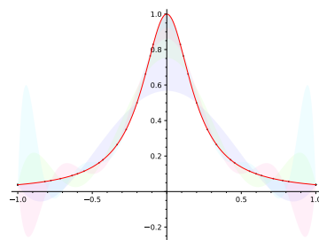
Figure 10.26 Sage polynomial approximations of f(x) = 1/(1 + 25x^2)
