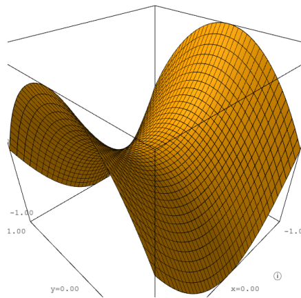
Figure 14.29 Sage+Jupyter iframe
