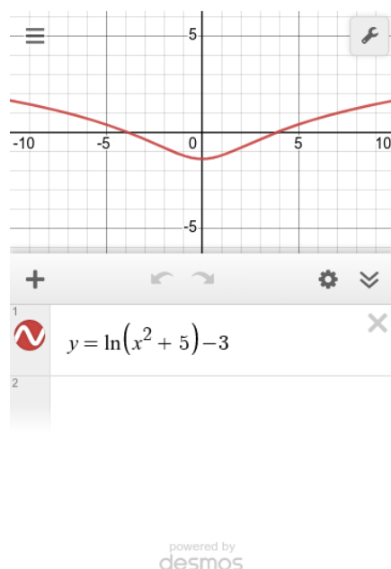
Figure 15.2 Graph of \ln(x^2 + 5) - 3
