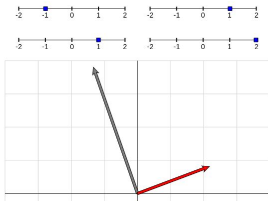
Figure 14.2 Eigenvector demonstration
