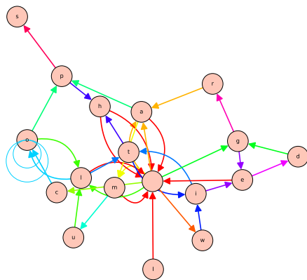
Figure 10.23 A Sage multigraph of a sentence
