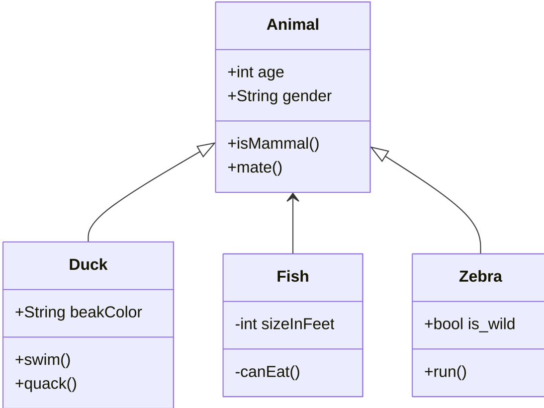
Figure 10.18 Mermaid Class Diagram
