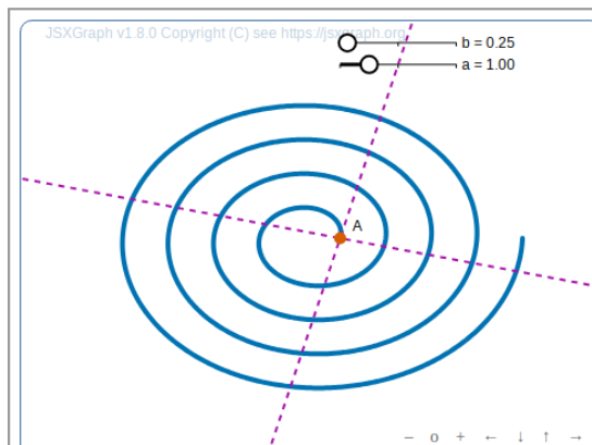
Figure 14.10 The Archimedean Spiral r = a + b\theta , 0 \leq \theta \leq 8\pi
