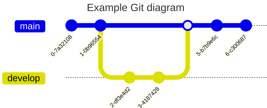
Figure 10.17 Mermaid Git Diagram
