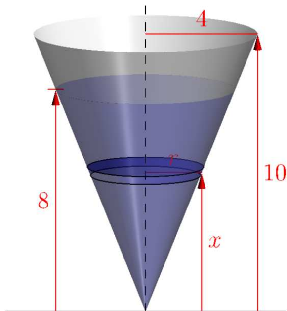
Figure 10.14 Work Cone (Asymptote Interactive 3D Image)
