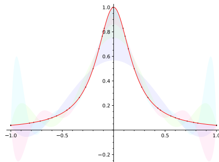
Figure 10.24 Sage polynomial approximations of f(x) = 1/(1 + 25x^2)
