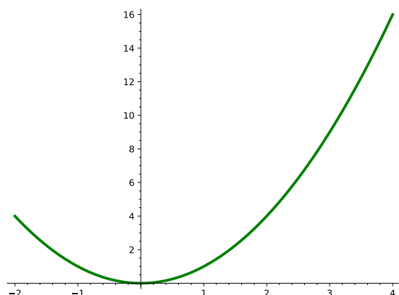
Figure 10.20 A Sage standard parabola, on [-2, 4]
