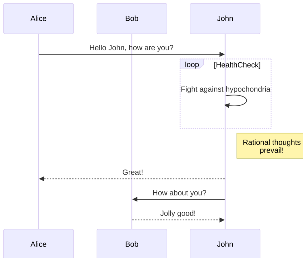
Figure 10.19 Mermaid Sequence Diagram
