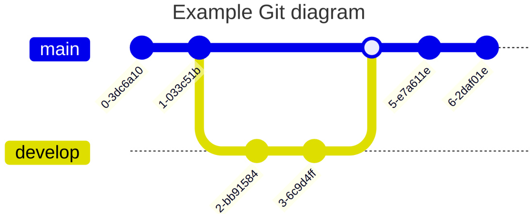
Figure 10.17 Mermaid Git Diagram
