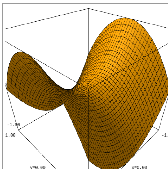
Figure 12.27 threejs saddle by Sage
