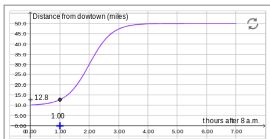
Figure 12.16 GeoGebra: modified material ID
