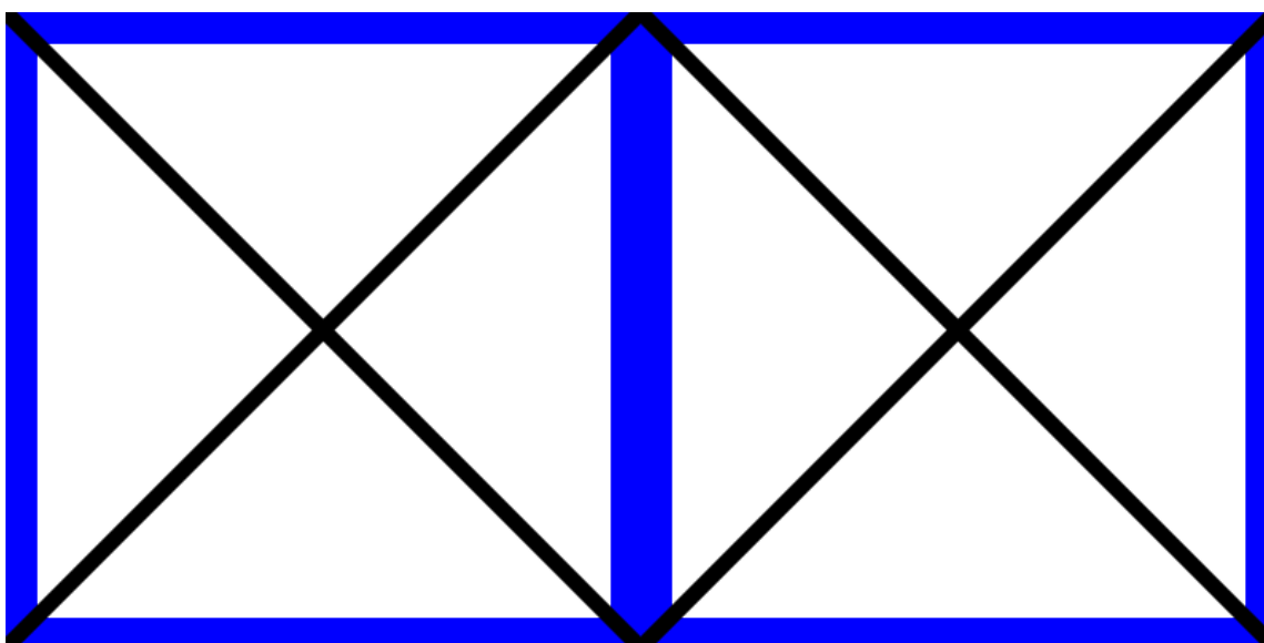
Figure 24.7 Two equally-spaced (identical) images
