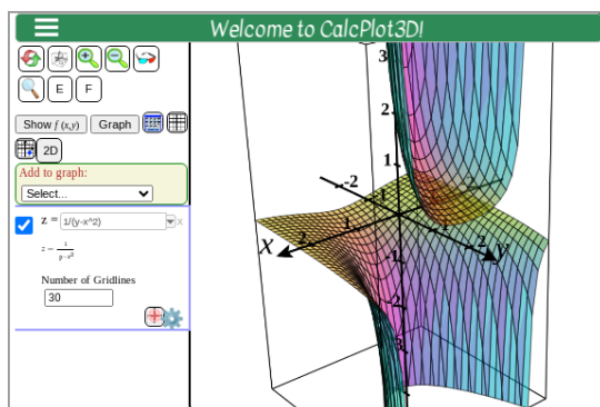
Figure 13.5 Plot of f(x, y) = \frac{1}{y - x^2} on [-2, 2] \times [-2, 2] (full application)
