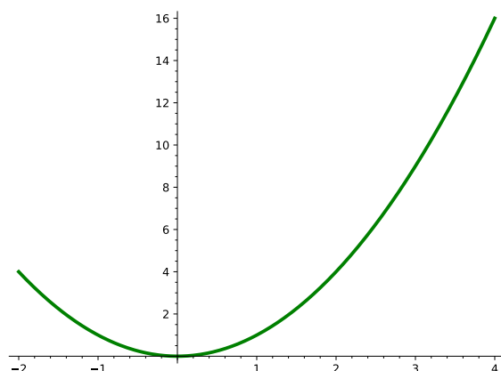
Figure 10.20 A Sage standard parabola, on [-2, 4]
