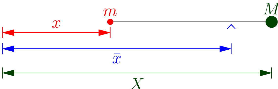
Figure 10.11 Asymptote Lever Demonstration
