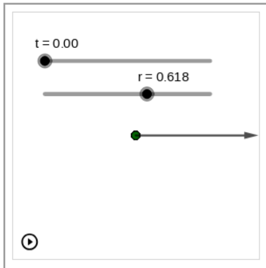
Figure 12.22 GeoGebra: from scratch
