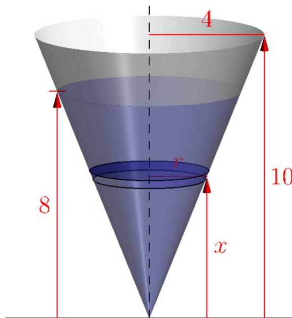
Figure 10.14 Work Cone (Asymptote Interactive 3D Image)
