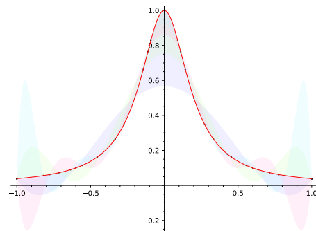
Figure 10.24 Sage polynomial approximations of f(x) = 1/(1 + 25x^2)
