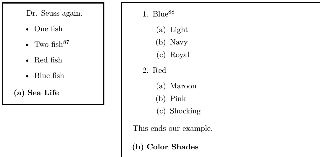
Figure 24.23 Two named lists
