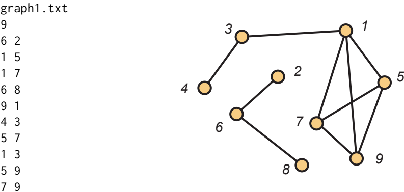
Figure 24.28 A graph defined by data (from Keller and Trotter’s Applied Combinatorics )
