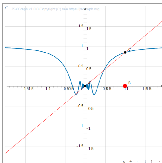
Figure 12.14 Graph of a function that is continuous but not differentiable at x = 0 because the slope of the secant line has no limit.
