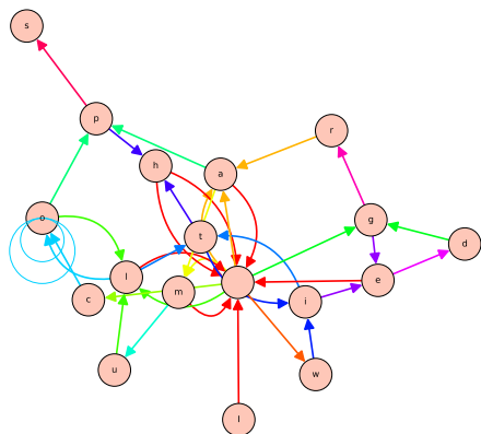
Figure 10.23 A Sage multigraph of a sentence
