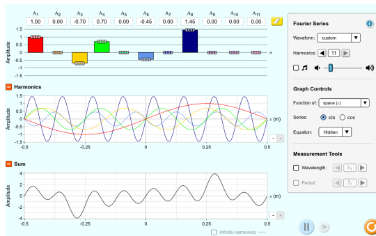
Figure 13.6 Fourier: Making Waves iframe
