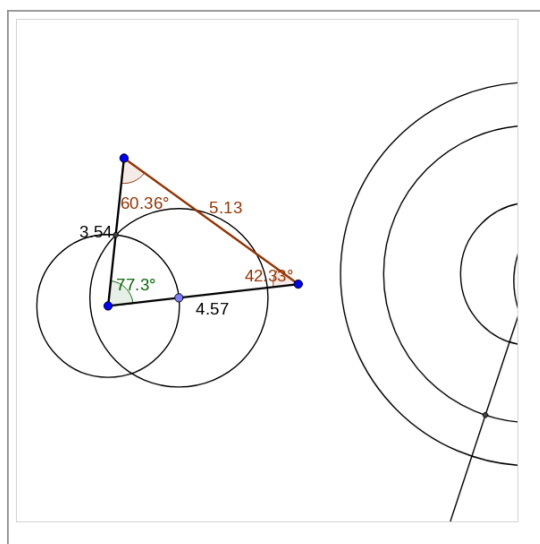
Figure 12.20 GeoGebra: a constructive “proof” that SAS congruence holds in Euclidean geometry (from Tevian Dray)
