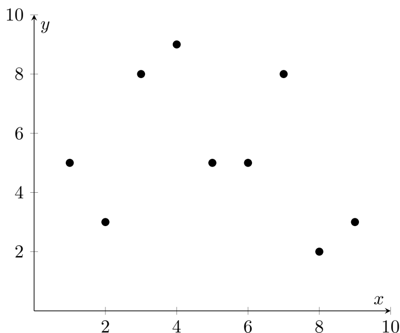
Figure 10.9 Full description with tabular
