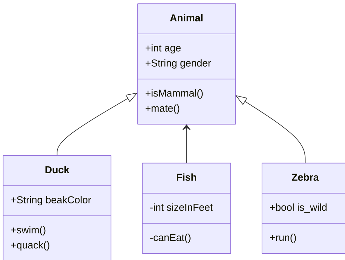
Figure 10.18 Mermaid Class Diagram
