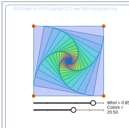
Figure 12.11 Infinity, from the JSXGraph Showcase
