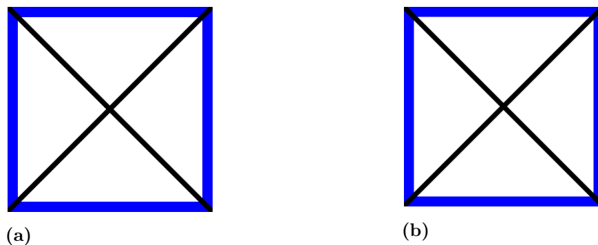
Figure 24.1 Side-by-Side, with figures as children, automatic margin
