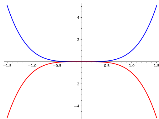
Figure 10.21 Two Sage plots on one set of axes
