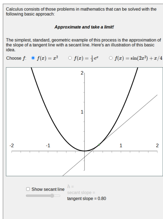
Figure 12.8 Tangent and secant slopes
