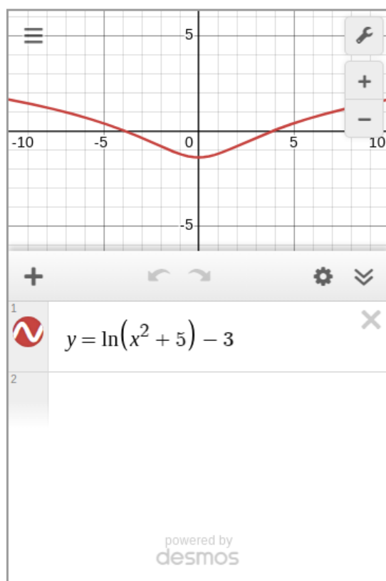
Figure 13.2 Graph of \ln(x^2 + 5) - 3
