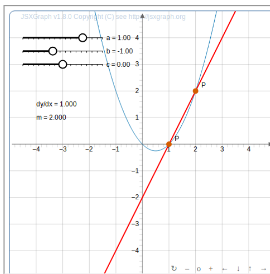
Figure 12.13 Finding the Tangent Line of a Quadratic Function
