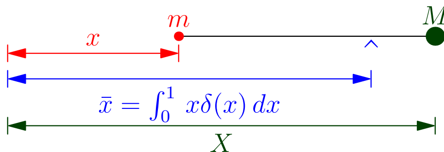
Figure 10.13 Asymptote Lever, plus Integral
