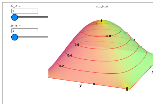
Figure 13.4 Probability wavefunction with contours (includes controls)
