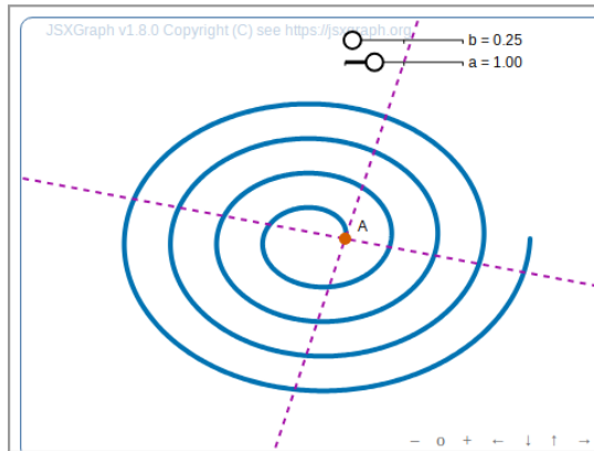
Figure 12.10 The Archimedean Spiral r = a + b\theta , 0 \leq \theta \leq 8\pi
