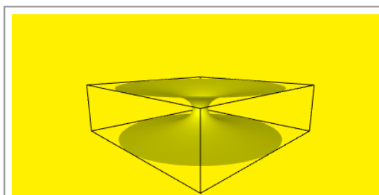
Figure 12.26 threejs catenoid surface, from n -Category Cafe
