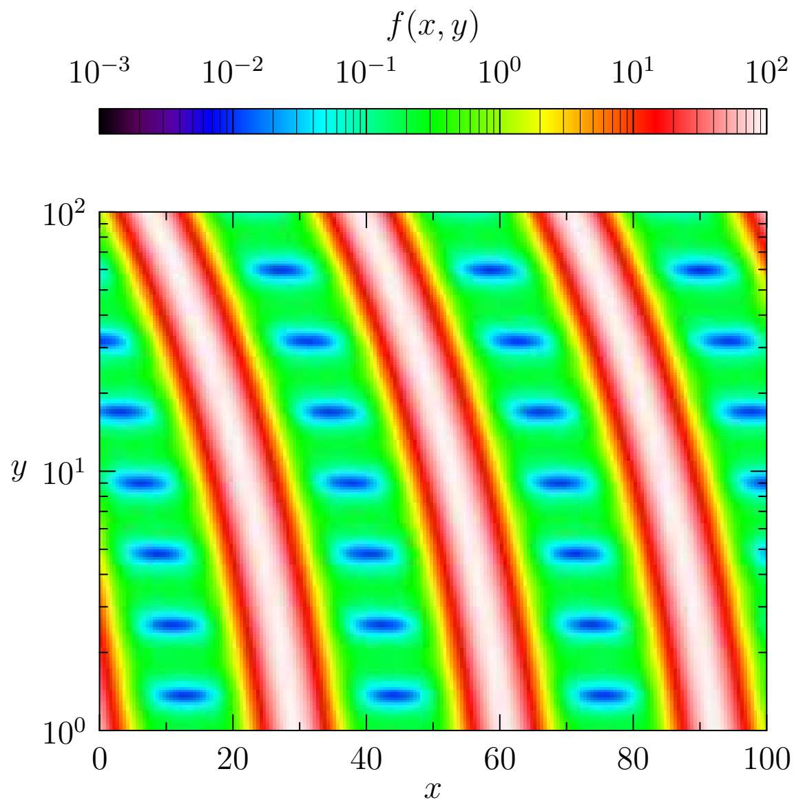
Figure 10.12 Asymptote Contour Plot
