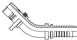
3C14 712 Plug-in koppling 45° R1/R2-slang
