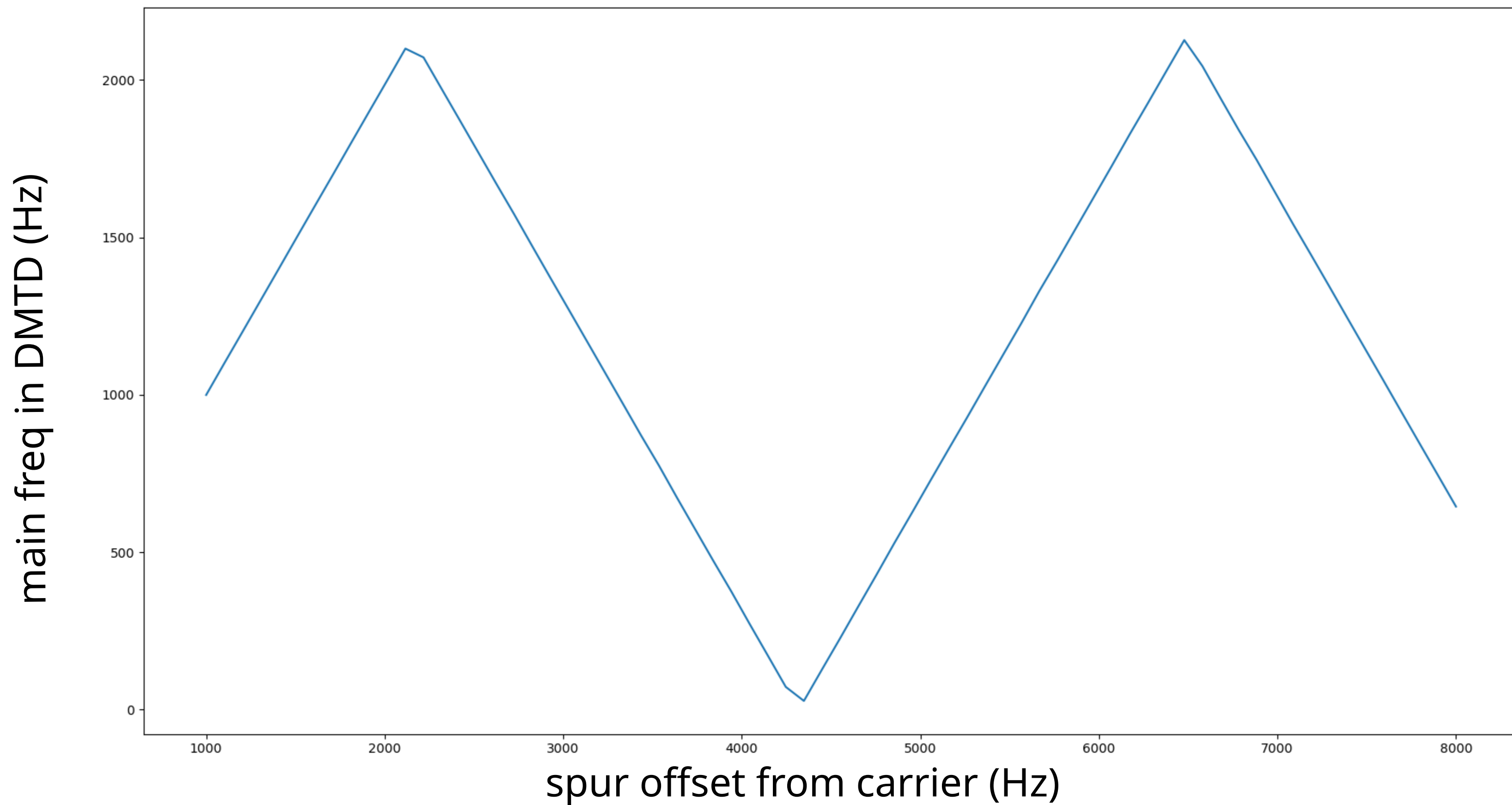
Dominant frequency in dmtdd output by spur offset
