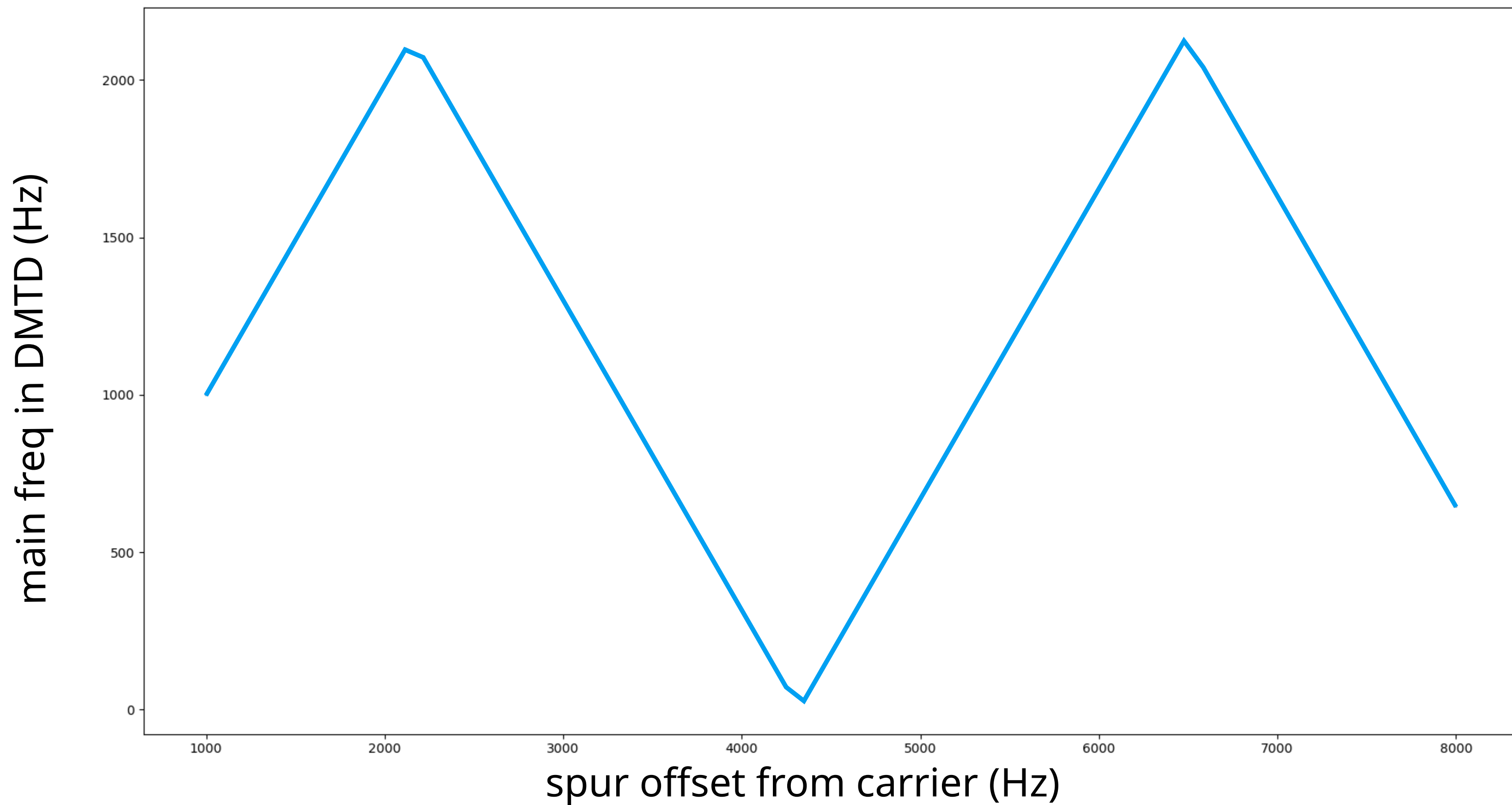
Dominant frequency in dmttd output by spur offset
