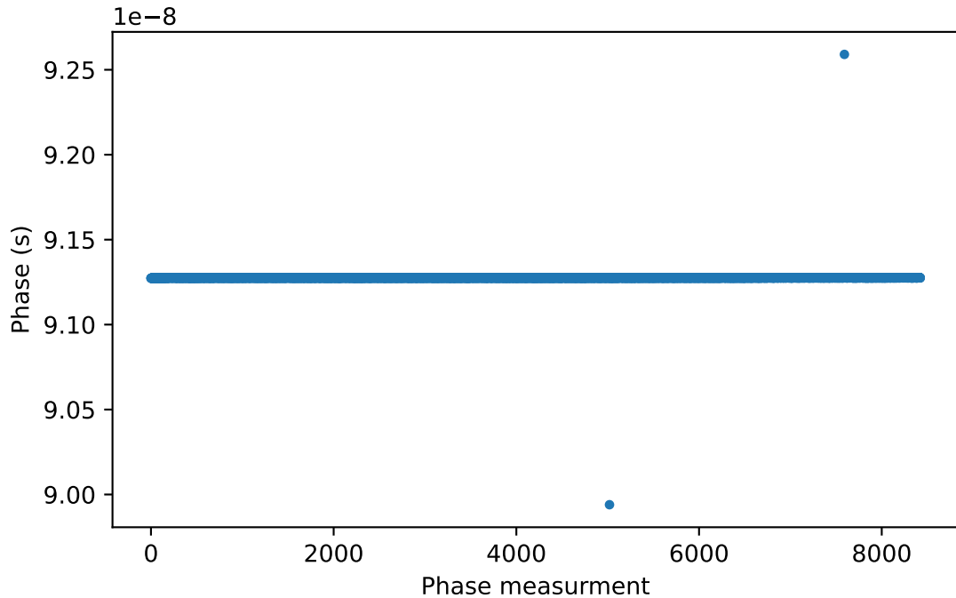
Repeated phase measurement of a clock against itself
