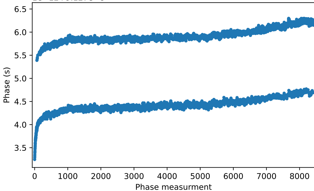
Repeated phase measurement of a clock against itself (zoom)
