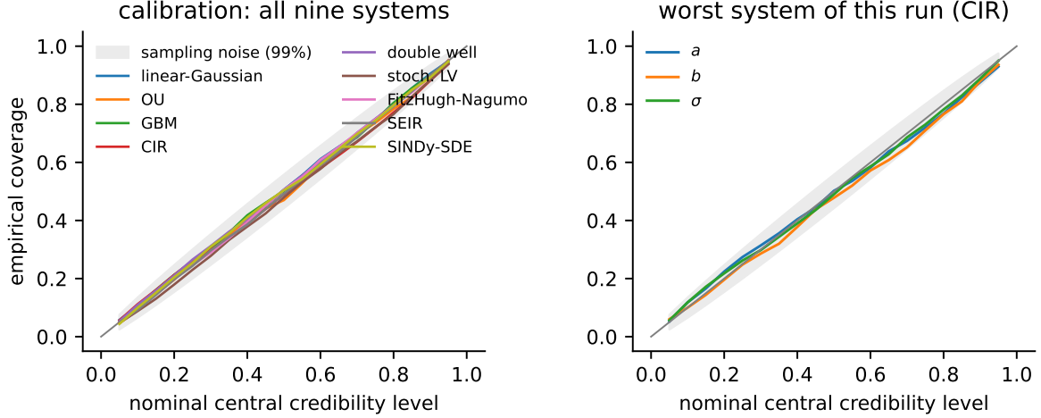
Figure 2: Calibration of the gallery models, read the way a practitioner would use them. Left: for each system, the fraction of the 500 test datasets in which the true parameter fell inside the posterior’s central q\% credible interval, plotted against q and averaged over the system’s parameters; a perfectly calibrated posterior follows the diagonal, and the gray band is the spread attributable to having only 500 datasets. All nine systems track the diagonal within the band. Right: the same curves for the individual parameters of the least calibrated system of this run (Cox–Ingersoll–Ross); the b curve shows the \approx 0.15 sd location shift discussed in the text. Rank-level detail for all 32 parameters is given in Appendix A (Fig. 8).
