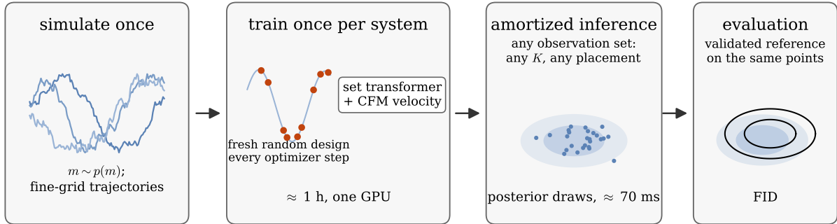
Figure 1: The approach. Parameters come from the prior and are simulated once on a fine grid (left). Training fits a conditional flow-matching posterior with a set-transformer encoder. Each optimizer step draws a fresh random observation design (Secs. 3, 4). The trained network returns posterior samples for any observation set of the experiment, with any number and any placement of points. We measure the accuracy against exact or validated reference posteriors computed on the same observed points (Sec. 5).
