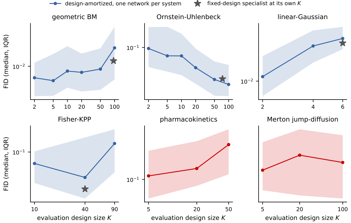
Figure 7: FID as a function of the evaluation design size, for one design-amortized network per system. The line is the median and the band is the interquartile range over the test observation sets of each bucket. A bucket has 100 sets for GBM, OU and linear-Gaussian, and 32 for the MCMC-referenced systems. Each set has a fresh random design and a per-design reference recomputed on exactly those points. These are the six systems whose references were built on a grid of design sizes. The rest of the suite has references at one design size (Table 2), which scores a model but does not trace a curve. Stars: networks of the same architecture trained on a single fixed design. They exist only at their own K and are shown for context. The Merton and pharmacokinetics curves use the converged references of Sec. 5.1. The text analyzes the pharmacokinetic rise with K , which is the precision floor. Both axes are logarithmic. Note the different vertical scales.
