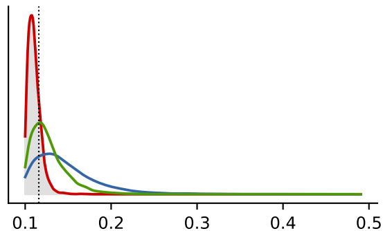
\sigma (volatility)
