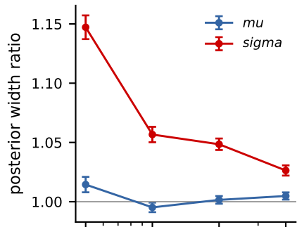
geometric BM (vs exact)
