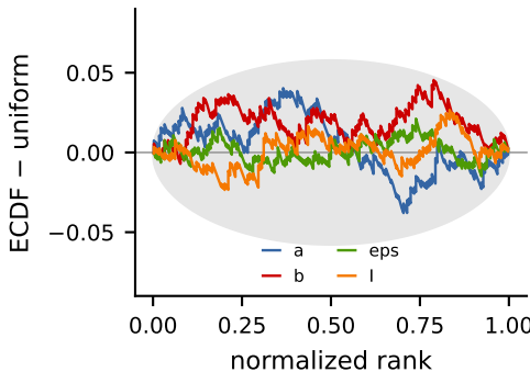
FitzHugh-Nagumo
