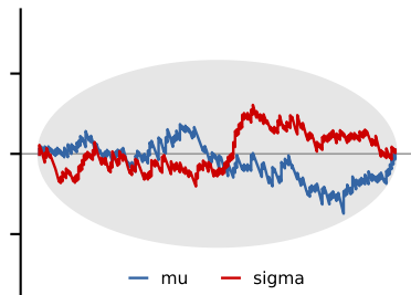
geometric BM
