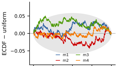
Cox-Ingersoll-Ross
