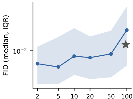
Fisher-KPP
