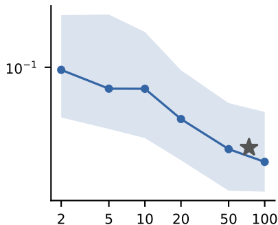
pharmacokinetics
