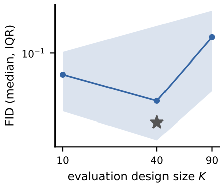
Fisher-KPP
