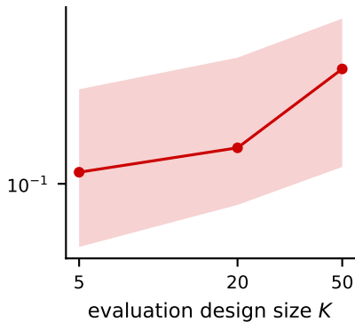
pharmacokinetics
