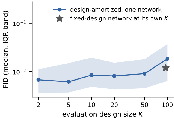
geometric BM (vs exact conjugate)
