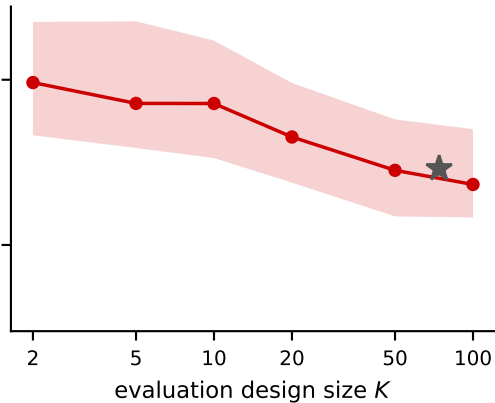
Ornstein-Uhlenbeck (vs exact-likelihood MCMC)
