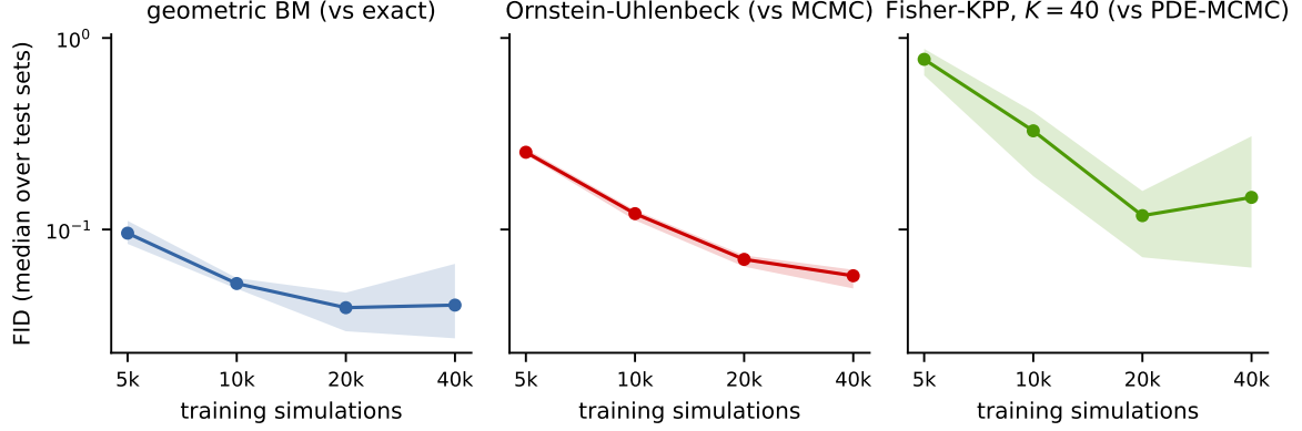
Figure 5: Convergence to the reference posterior with training budget: median FID (log scale) on three systems over budgets of 5,000–40,000 simulations with optimizer steps scaled proportionally. Lines: mean over three independent training seeds; shaded bands: seed range. The widening Fisher–KPP band at large budgets is the seed-level freedom of the weakly identified ridge direction discussed in the text. References: exact conjugate posterior (GBM), exact-likelihood MCMC (OU), PDE-likelihood MCMC (Fisher–KPP, fixed K = 40 design).
