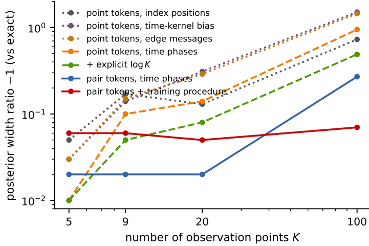
Figure 3: The data of Table 5 in graphical form: excess posterior width for the GBM volatility — the width ratio against the exact posterior minus one, so 0.1 means a posterior 10% too wide and lower is better — as a function of the number of observation points K (both axes logarithmic). Dotted curves: point-token variants with no set-size information, which degrade as designs become dense; dashed: partial repairs; solid: increment tokens, and increment tokens combined with the training procedure of Sec. 5, which is flat in K .
