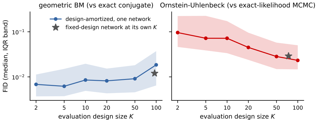
Figure 2: The data of Table 4 with distributional detail: median FID (line) and interquartile range (band) over 100 test observation sets per design-size bucket, for one design-amortized network per system evaluated with a fresh random design and an exact per-design reference for every test set. The star is the fixed-design network of the same architecture and simulation budget, which exists only at its own K . Both axes logarithmic.
