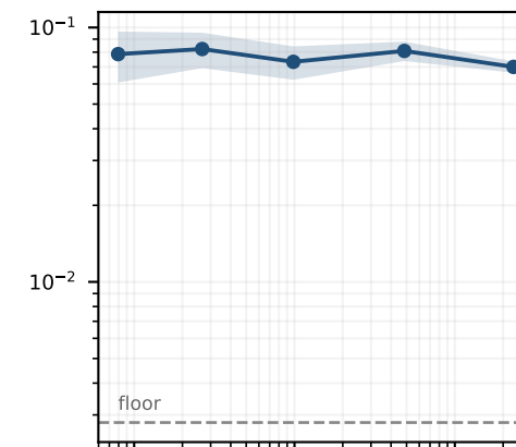
Fisher-KPP
