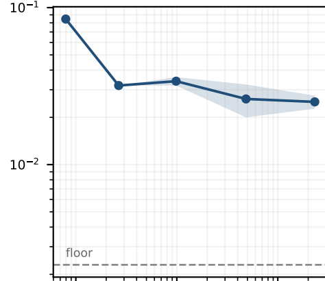
Heston
