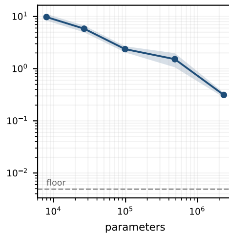
Hodgkin-Huxley
