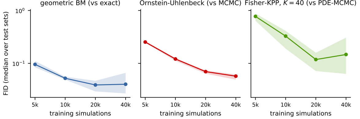
Figure 3: Convergence to the reference posterior with training budget: median FID (log scale) on three systems over budgets of 5,000–40,000 simulations with optimizer steps scaled proportionally. Lines: mean over three independent training seeds; shaded bands: seed range. The widening Fisher–KPP band at large budgets is the seed-level freedom of the weakly identified ridge direction discussed in the text. References: exact conjugate posterior (GBM), exact-likelihood MCMC (OU), PDE-likelihood MCMC (Fisher–KPP, fixed K = 40 design).
