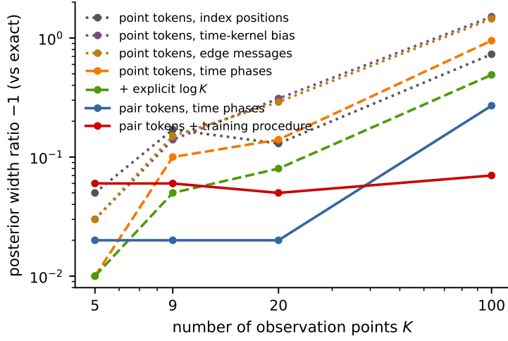
Figure 4: The data of Table 7 in graphical form: excess posterior width for the GBM volatility — the width ratio against the exact posterior minus one, so 0.1 means a posterior 10% too wide and lower is better — as a function of the number of observation points K (both axes logarithmic). Dotted curves: point-token variants with no set-size information, which degrade as designs become dense; dashed: partial repairs; solid: increment tokens, and increment tokens combined with the training procedure of Sec. 5, which is flat in K .
