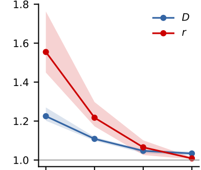
Fisher-KPP, K = 40 (vs PDE-MCMC)
