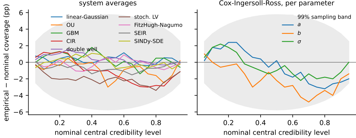
Figure 2: Empirical coverage of central credible intervals for the fixed-design gallery, shown as the deviation from the nominal level. For each system, 500 synthetic datasets are simulated with known parameters and the posterior’s central q\% interval is checked against the truth; a calibrated posterior has zero deviation at every level, and the gray band is the 99% pointwise range induced by the finite number of test datasets. Left: deviation averaged over each system’s parameters. Right: individual parameters of Cox–Ingersoll–Ross, the system with the largest deviation in this run; the b curve reflects the \approx 0.15 sd location shift discussed in the text. Rank-level detail for all 32 parameters is in Appendix A (Fig. 8).
