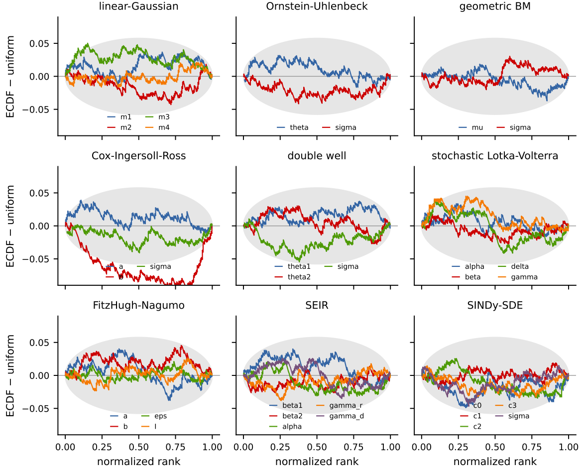
Figure 8: Calibration check for the fixed-design gallery. Procedure: for each system, 500 synthetic datasets are simulated with known parameters; for each dataset the model produces 200 posterior draws, and the rank of the true parameter among the draws is recorded. If the posterior is calibrated, these ranks are uniform. Each curve shows, for one parameter, the deviation of the empirical CDF of normalized ranks from the uniform diagonal; the gray band is the 99% range attributable to sampling noise at 500 datasets. A curve bulging below zero on the left indicates a posterior shifted low relative to the truth, and vice versa. All curves stay within the band except Cox–Ingersoll–Ross b , whose deviation corresponds to the \approx 0.15 sd location shift discussed in the text.
