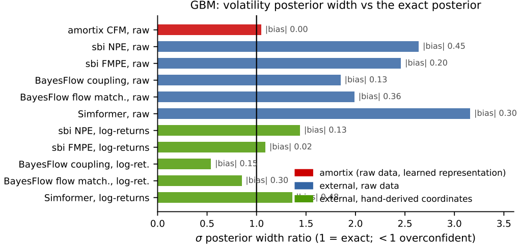
Figure 6: The accuracy axis of Tables 4 and 5 at a glance: volatility posterior width as a ratio to the exact posterior, so 1 is exact, larger is too wide, and values below one are overconfident. Annotations give the absolute posterior-mean bias in units of the exact posterior standard deviation.
