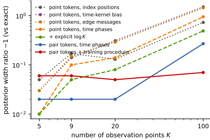
Figure 7: The data of Table 8 in graphical form: excess posterior width for the GBM volatility — the width ratio against the exact posterior minus one, so 0.1 means a posterior 10% too wide and lower is better — as a function of the number of observation points K (both axes logarithmic). Dotted curves: point-token variants with no set-size information, which degrade as designs become dense; dashed: partial repairs; solid: increment tokens, and increment tokens combined with the training procedure of Sec. 5, which is flat in K .
