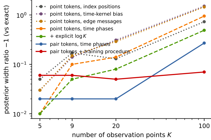
Figure 5: The data of Table 6 in graphical form: excess posterior width for the GBM volatility — the width ratio against the exact posterior minus one, so 0.1 means a posterior 10% too wide and lower is better — as a function of the number of observation points K (both axes logarithmic). Dotted curves: point-token variants with no set-size information, which degrade as designs become dense; dashed: partial repairs; solid: increment tokens, and increment tokens combined with the training procedure of Sec. 5, which is flat in K .
