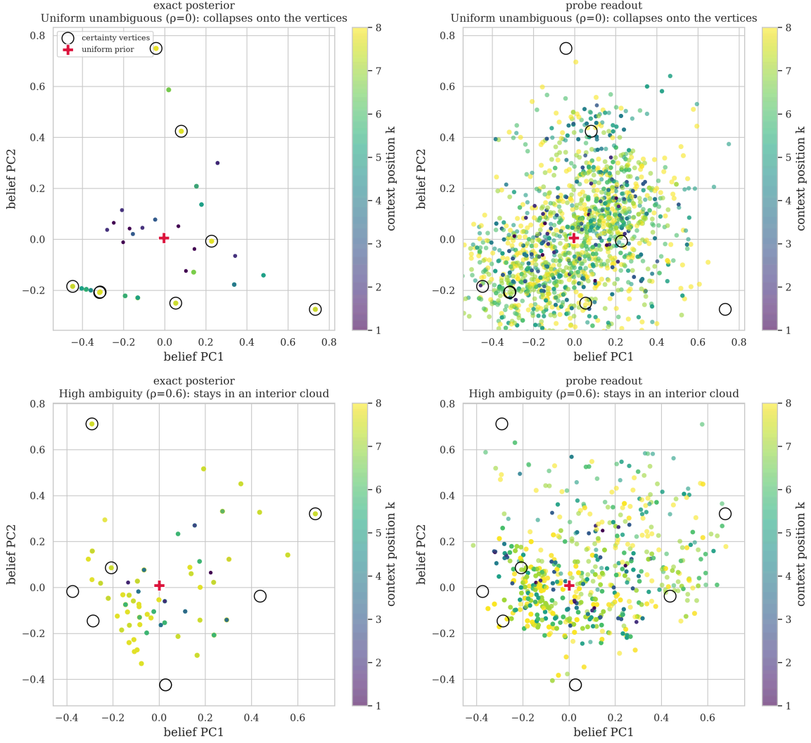
Figure 10: Exact posterior (left column) and linear-probe readout (right column) in belief-PCA, colored by context position k (marker size grows with k ), for the uniform corner \rho = 0 (top) and the high-ambiguity corner \rho = 0.6 (bottom). Open black circles mark the eight certainty vertices (one-hot roots) and the red + the uniform prior, both projected into the panel’s own basis (the circles are hollow so the points landing inside them stay visible). Because root-class labels are not aligned across grammars, each row keeps its native belief-PCA basis and axis limits are shared only within a row; the vertex markers give the label-agnostic reference. At \rho = 0 the late-context beliefs land on the vertices (collapse to certainty); at \rho = 0.6 they stay in an interior cloud near the prior, off the vertices (non-collapse) — and the probe readout occupies the same region as the exact posterior.
